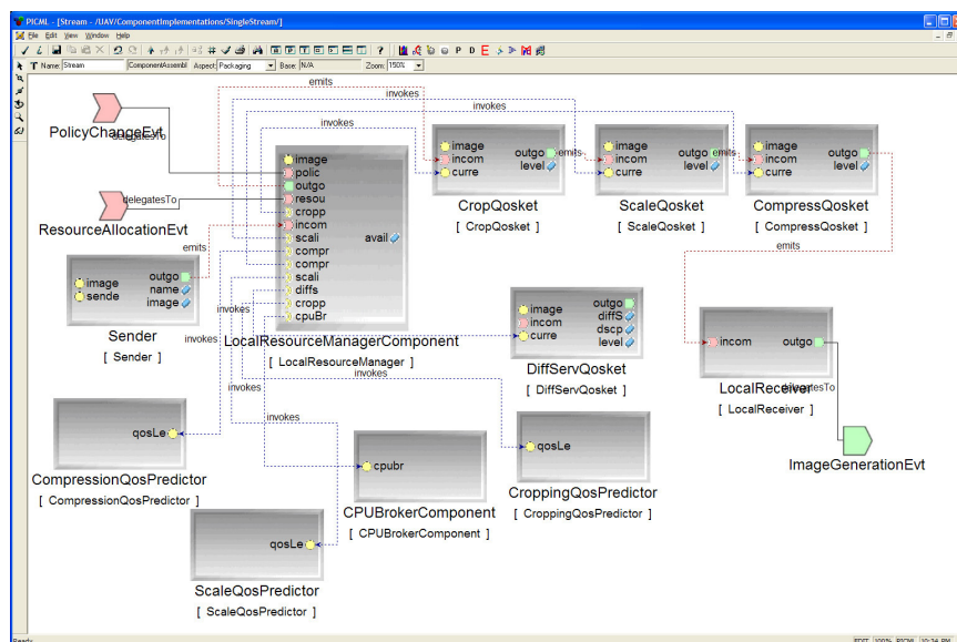
Fig. 3. Interaction Definition
