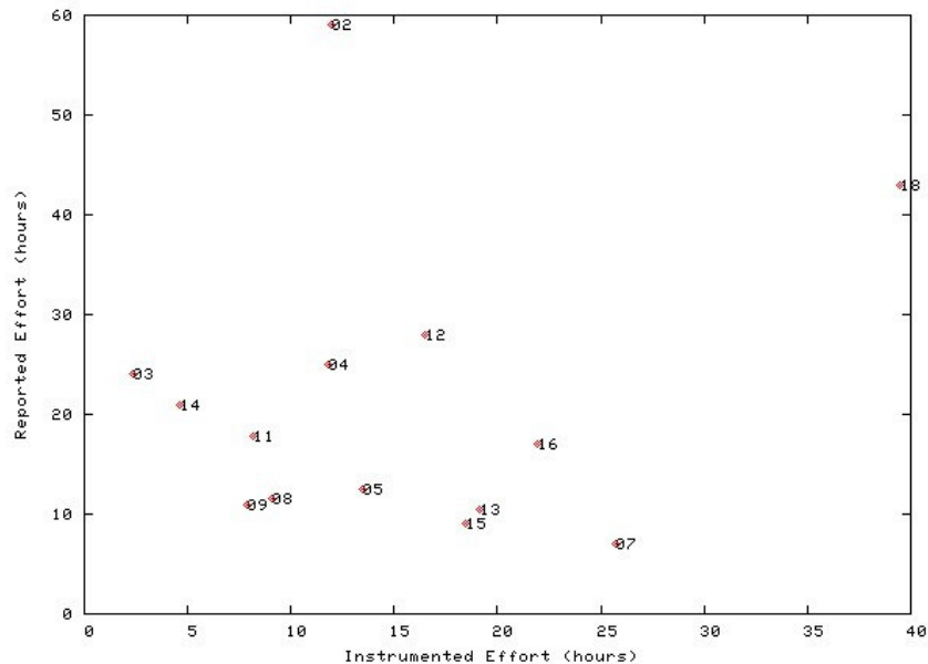
Figure 5 – Reported Effort vs. Instrumented Effort
