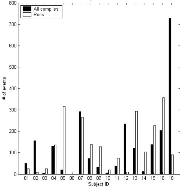
Figure 1 – Compiles vs. Runs
